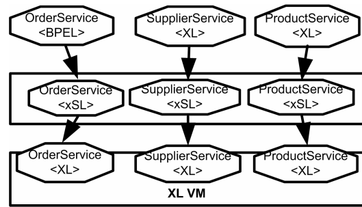
Figure 8: Scenario II – All XL
