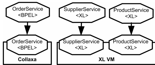
Figure 7: Scenario I – Traditional; BPEL and XL
