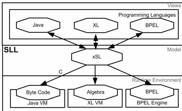
Figure 1: The Service Language Layer (SLL)
