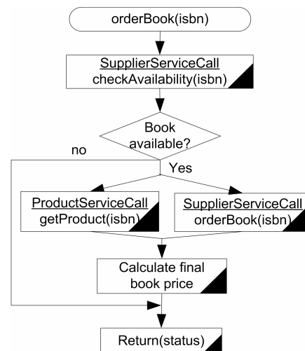
Figure 6: The orderBook operation workflow
