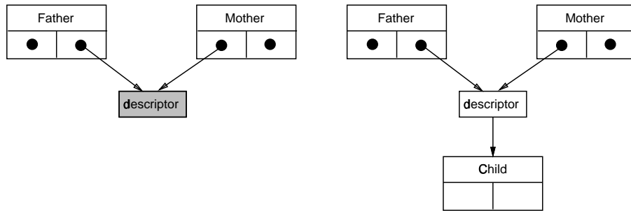
Figure 3: The Scenario of Indirect Swizzling
