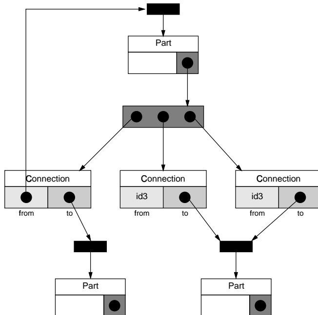
Figure 10: Context-Specific Swizzling in the OO1 Benchmark
