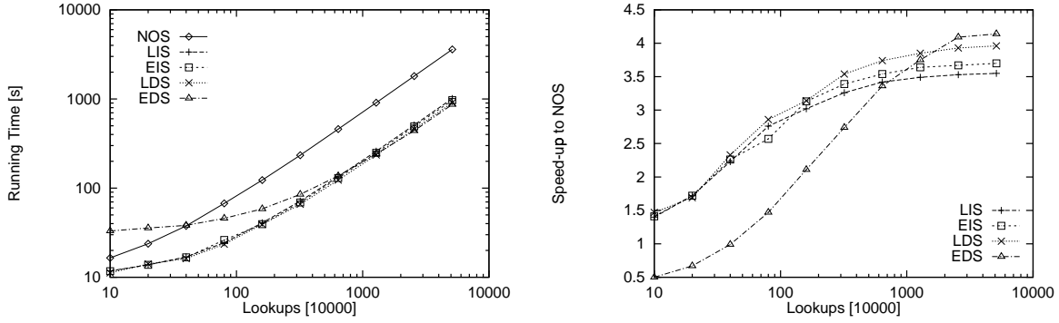
Figure 12: Measuring the Lookup Operation
