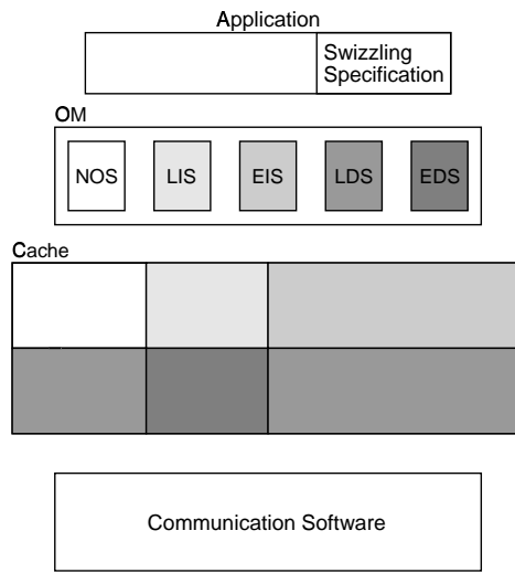
Figure 6: Granularities of Adaptable Pointer Swizzling
