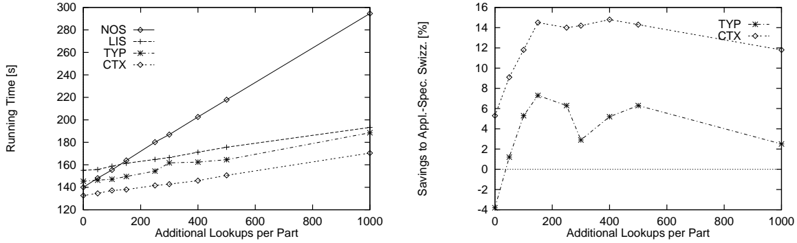
Figure 14: Traversals in Combination with Lookups (warm)
