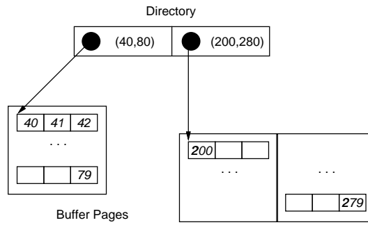
Figure 5: The Directory of a List
