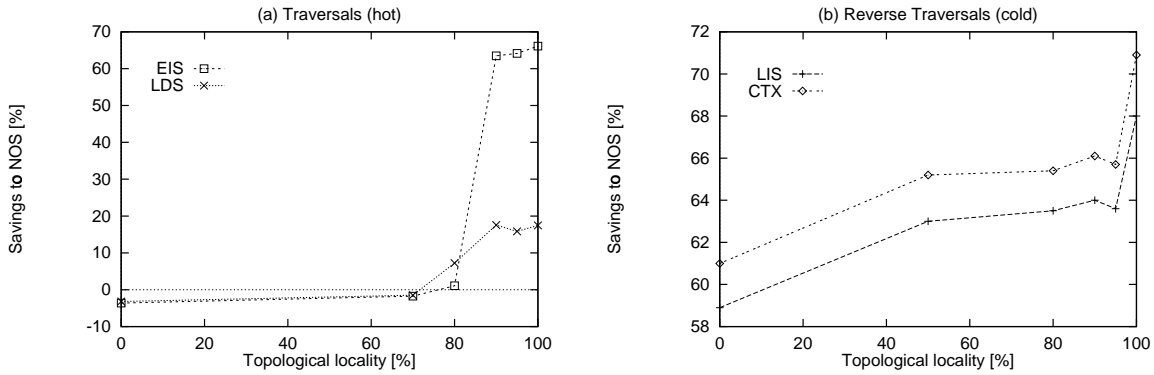
Figure 17: Varying Topological Locality
