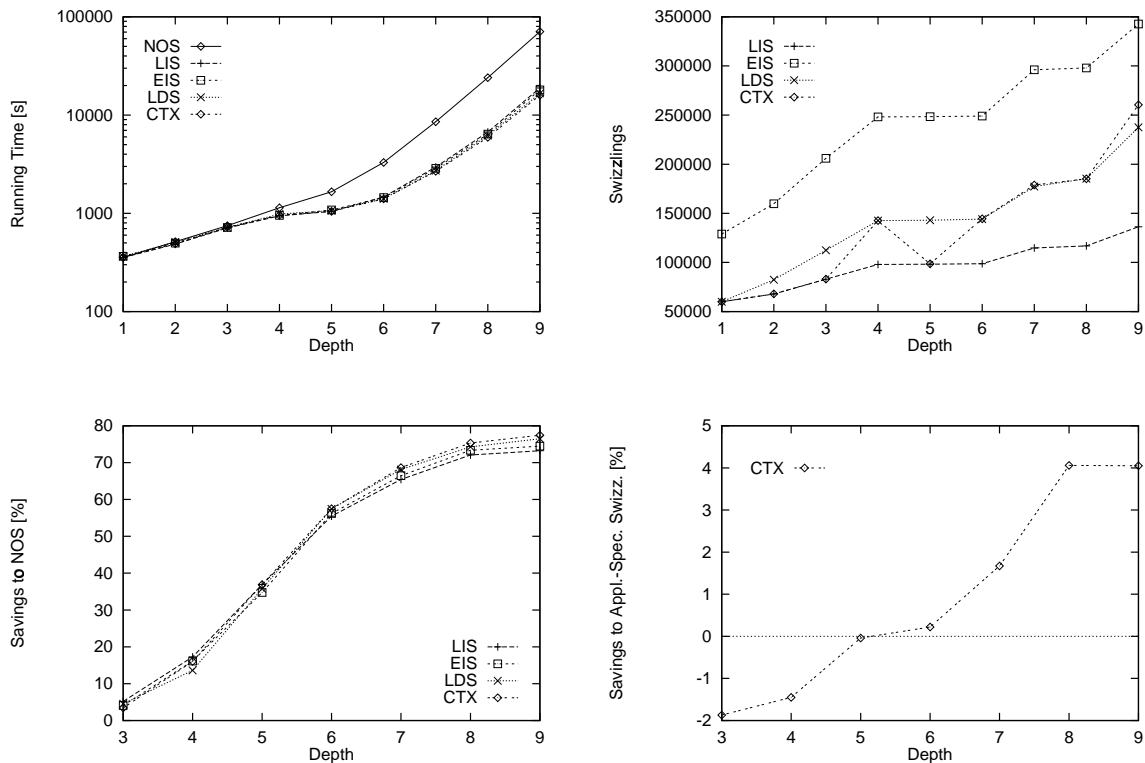
Figure 15: Measuring Reverse Traversals
