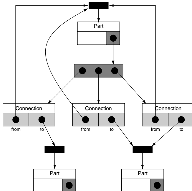
Figure 9: Type-Specific Swizzling in the OO1 Benchmark
