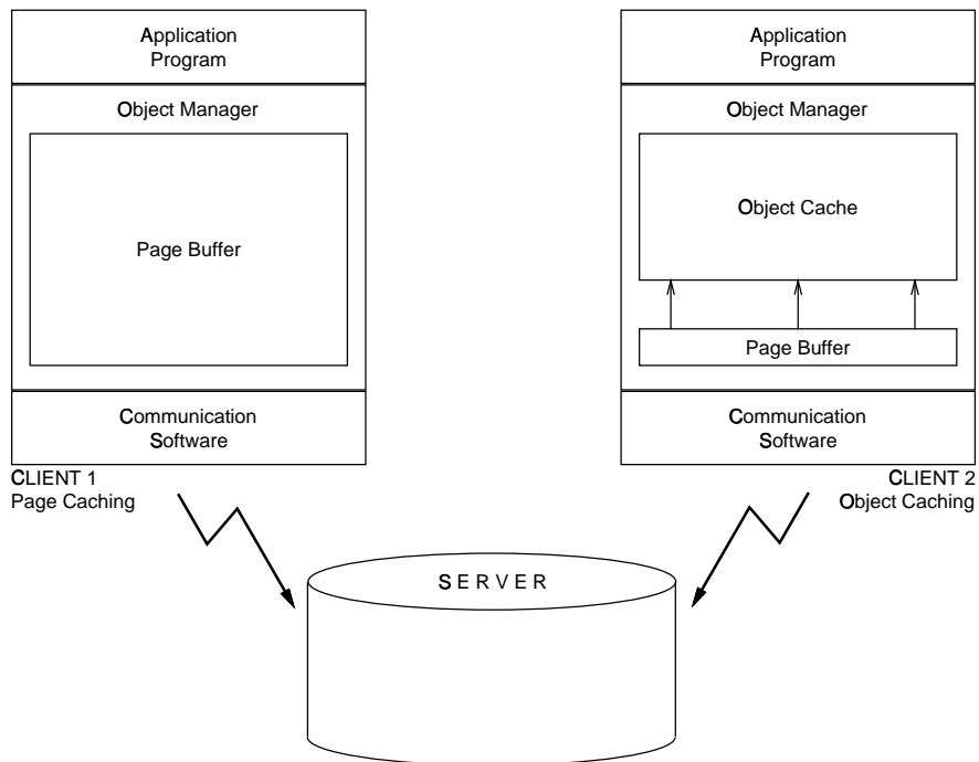
Figure 1: Architecture of an Object Base System
