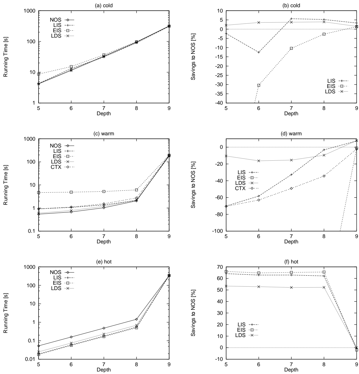
Figure 13: Measuring Traversals
