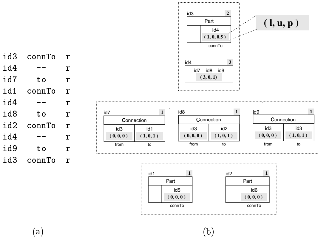
Figure 20: Generating a Swizzling Graph (b) from an Object Trace (a)
