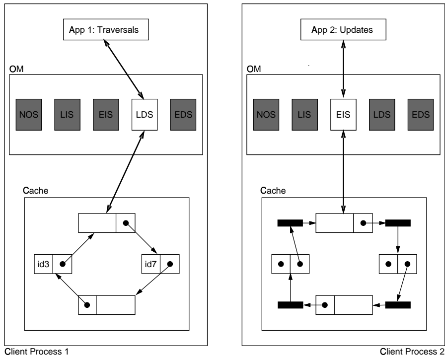
Figure 8: The Scenario of Application-Specific Swizzling
