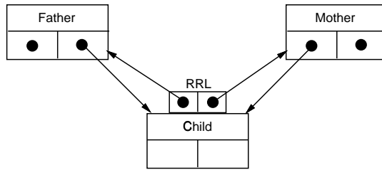
Figure 2: Direct Swizzling and an RRL
