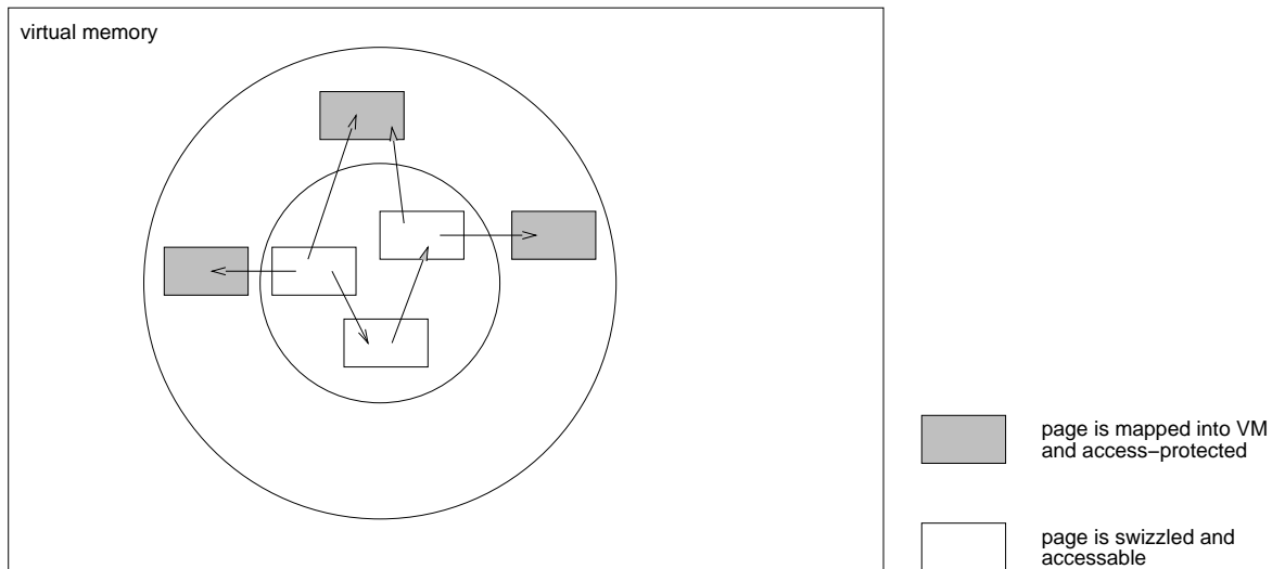
Figure 4: Wave Front of Swizzled and Mapped Pages in the Texas Persistent Store
