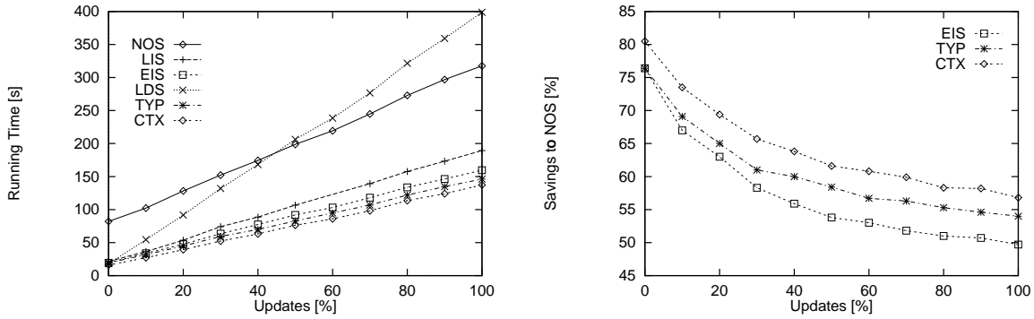
Figure 16: Operation Mix: Updates and Lookups (hot)
